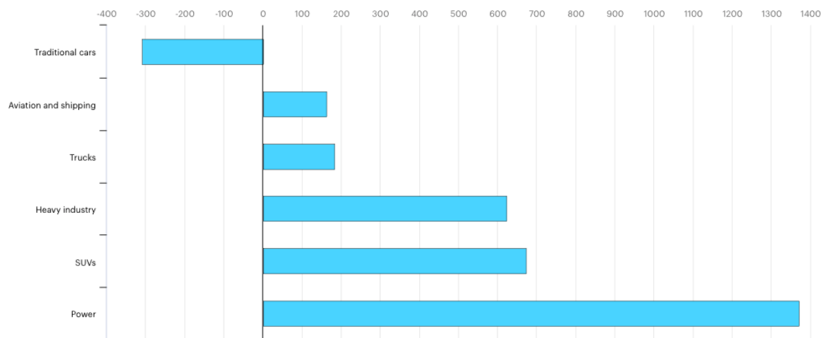
Figure 7 IEA, Growth in CO 2 emissions by energy sub-sector from 2010 to 2021, IEA, Paris https://www.iea.org/data-and-statistics/charts/growth-in-CO 2 -emissions-by-energy-sub-sector-from-2010-to-2021
